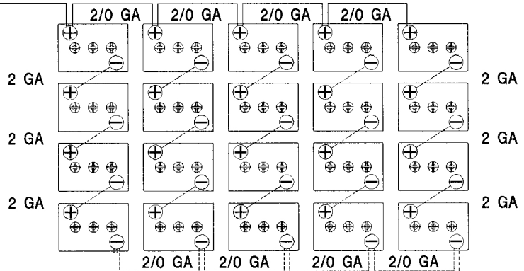
BATTERY BANK 1125A-H @ 24 VDC
